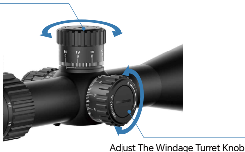
Capped Resettable to Zero Elevation Turret Knob
