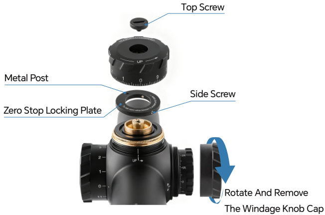
Capped Resettable to Zero Elevation Turret Knob
